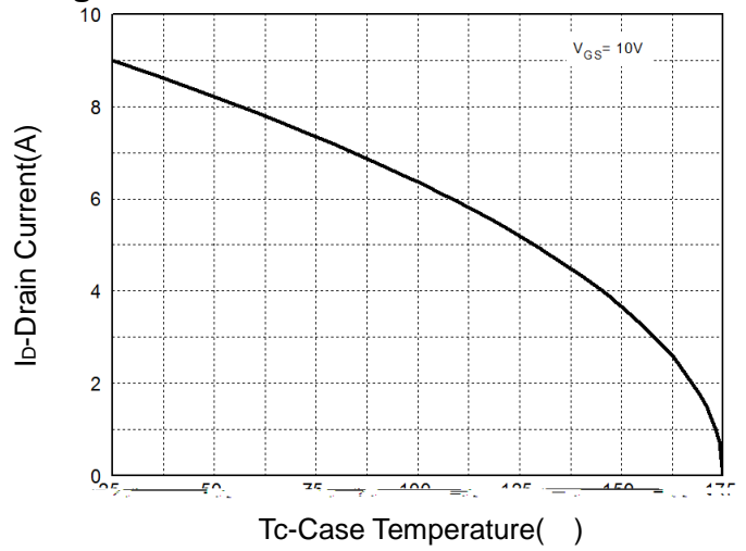
Figure 2: Drain Current
